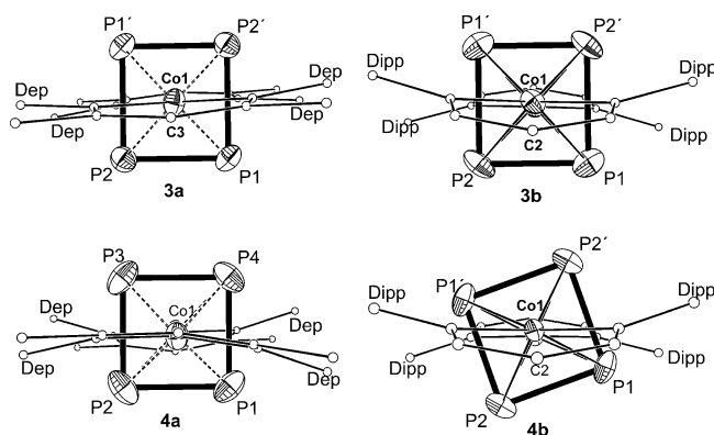
Figure 4. The \text{Co}_2\text{P}_4 cores viewed along \text{Co1}–\text{Co1}' in the molecular structure of 3a , 4a , 3b , and 4b . Selected distances ( \text{\AA} ) and angles ( ^\circ ) for 4a : \text{Co1}–\text{P1} 2.3740(9), \text{Co1}–\text{P4} 2.3747(8), \text{Co1}–\text{P2} 2.3750(9), \text{Co1}–\text{P3} 2.3814(9), \text{Co2}–\text{P2} 2.3577(9), \text{Co2}–\text{P3} 2.3986(9), \text{Co2}–\text{P4} 2.4084(9), \text{P1}–\text{Co2} 2.3495(9), \text{P1}–\text{P2} 2.163(1), \text{P1}–\text{P4} 2.225(1), \text{P2}–\text{P3} 2.230(1), \text{P3}–\text{P4} 2.154(1), \text{P2}–\text{P1}–\text{P4} 90.12(4), \text{P1}–\text{P2}–\text{P3} 89.64(4), \text{P4}–\text{P3}–\text{P2} 90.23(4), \text{P3}–\text{P4}–\text{P1} 90.01(4). Selected distances ( \text{\AA} ) and angles ( ^\circ ) for 4b : \text{Co1}–\text{P1} 2.3734(5), \text{Co1}–\text{P2} 2.3751(5), \text{Co1}–\text{P1}' 2.3768(5), \text{Co1}–\text{P2}' 2.4046(5), \text{P1}–\text{P2} 2.1739(7), \text{P1}–\text{P2}' 2.1976(7), \text{P2}–\text{P1}–\text{P2}' 90.85(2), \text{P1}–\text{P2}–\text{P1}' 89.15(2). Ellipsoids at 50% probability level.
